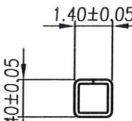
SEC. C-C
