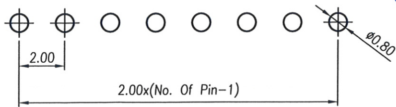
RECOMMENDED P.C.B LAYOUT (TOLERANCE:±0.05)
