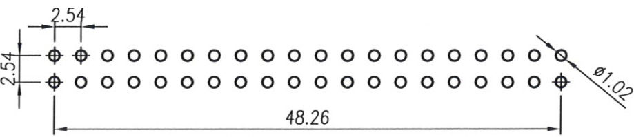
RECOMMENDED PCB LAYOUT (TOLERANCE:±0.05)
