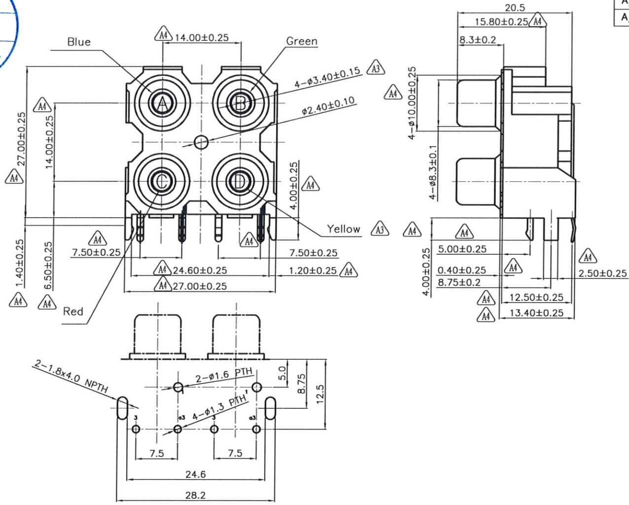
P.C.B LAYOUT BOTTOM VIEW
